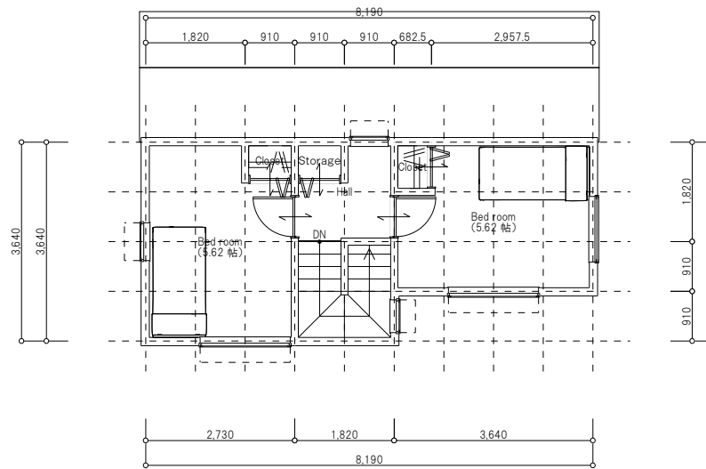
3rd FLOOR PLAN
